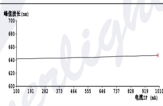
Spectral wavelength
