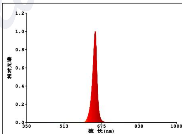
Spectral wavelength
